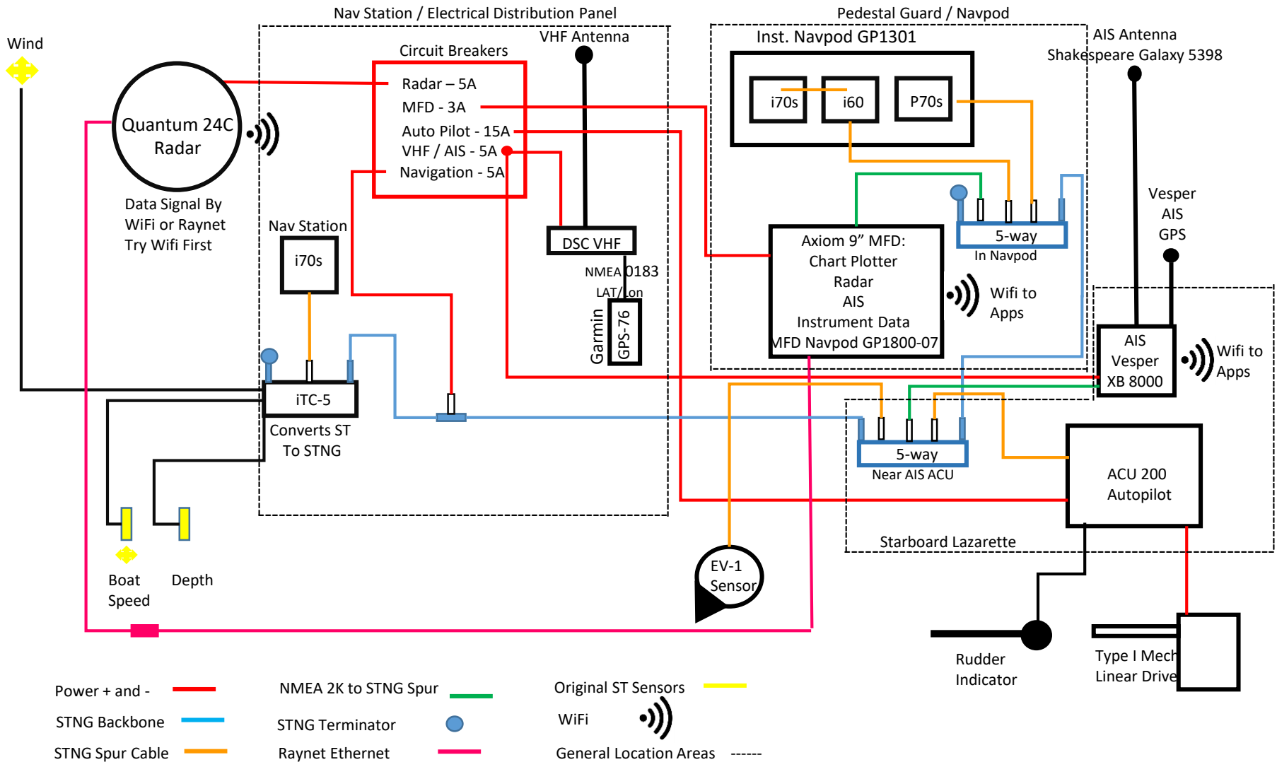
Raymarine Upgrade Schematic – 5/12/2018
