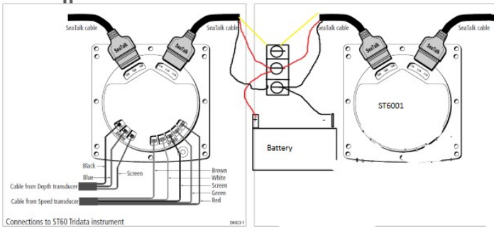
Connections to ST60 Tridata instrument
