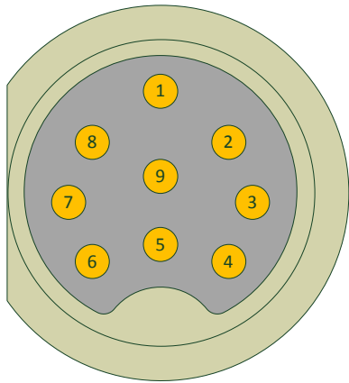
View of bulkhead connector from outside of the product
